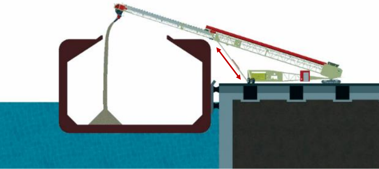
Telescopic fully raised and extended c/w 360 degree trimmer chute
